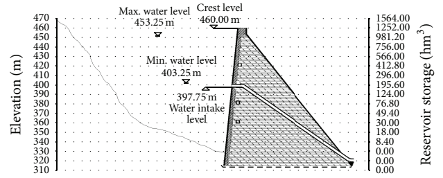
FIGURE 1: Cross-sectional view of Adiguzel reservoir.
